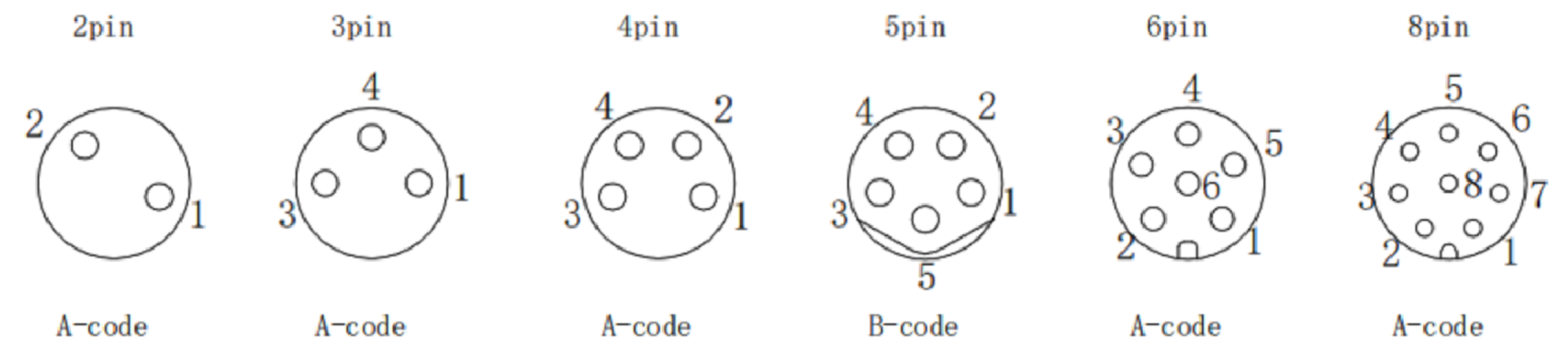
Pin assignment front view/针位分布前视图
